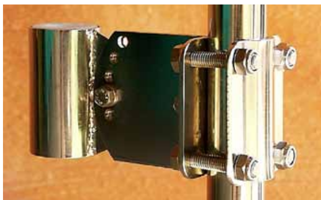
Rail fitting for Gangway (V4A) Attaches to all rails up to 30 mm diameter
